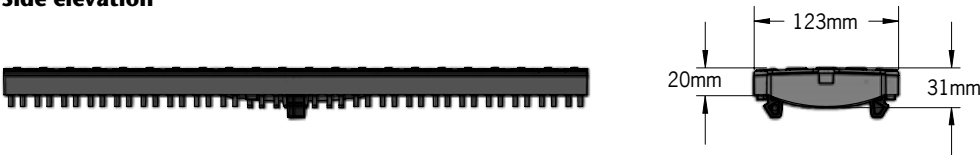
Side elevation
