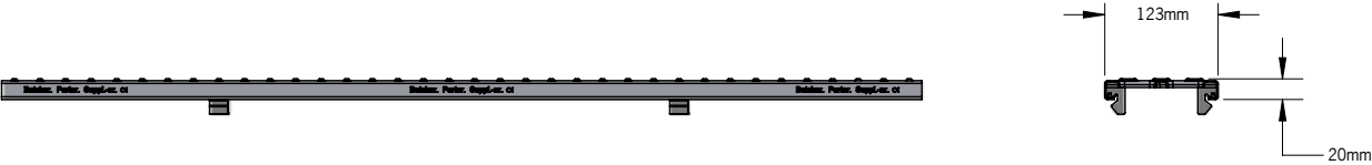
Side elevation
