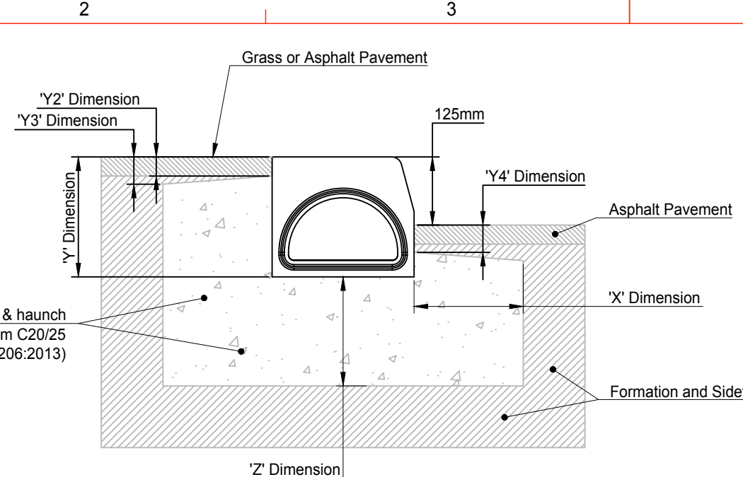
1 : 10 ACO KerbDrain KDHB Grass or Asphalt Pavement
