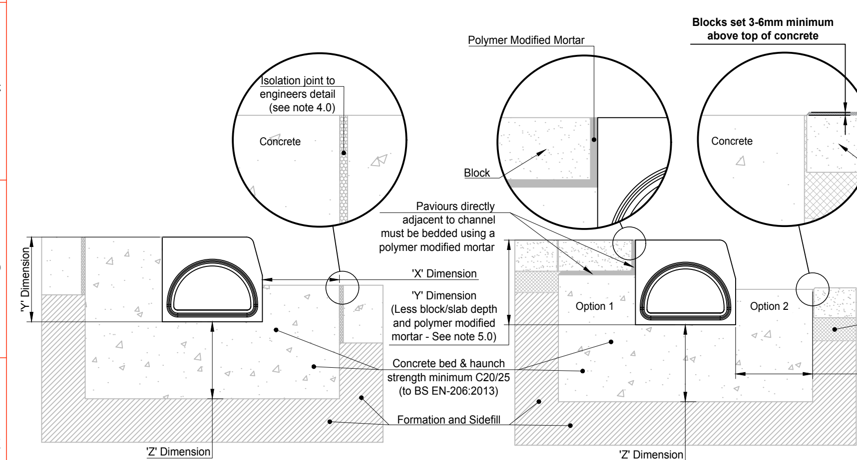
1 : 10 ACO KerbDrain KDHB Concrete Pavement
