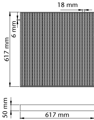
Stainless 5 Star grate
