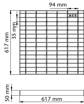
Galvanised Transverse grate
